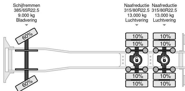
Volvo FH 16.650 | 6X4 + 6X2 | TANDEMLIFT | VDS | RETAR...
