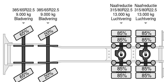
Scania R580 V8 NGS | 8X4 | BIG AXLES | RETARDER | 44 ...
