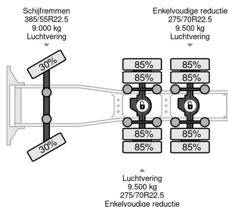
Scania R580 V8 NGS | 6X4 | RETARDER | HYDRAULICS | 66...
