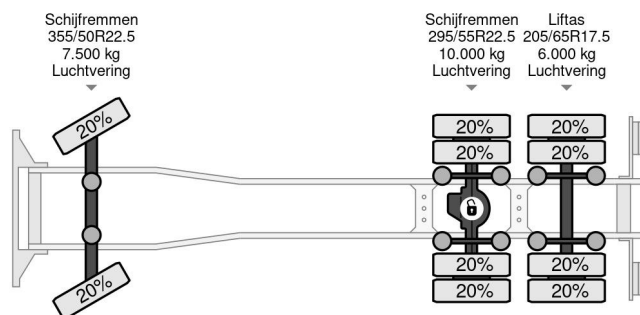
Scania R450 | 6X2 | GS MEPEL | TRUCK TRANSPORTER | ...
