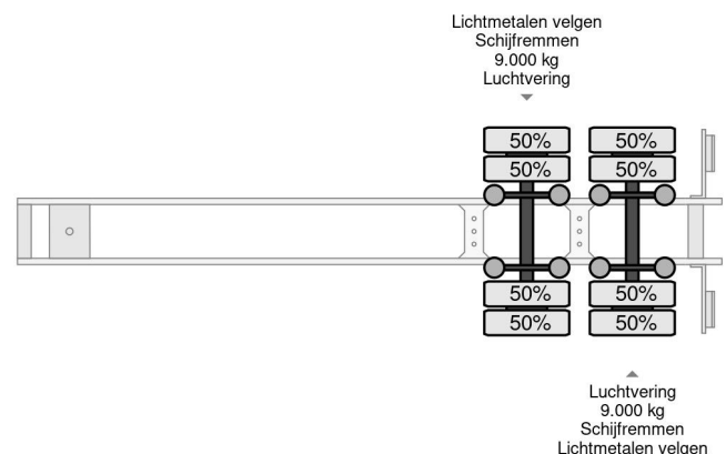
Meusburger MPG-2 | 2-AXLE | HYDR HEBEDACH / SCHIEB...
