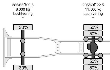
DAF XF 480 | 4X2 | LOWDECK | 2X TANK | PARKING AIRCO
