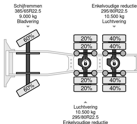
Volvo FH 540 | 6X4 - 6X2 | TANDEMLIFT | 70 TON | HYDR | ...
