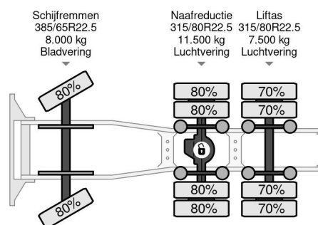
Volvo FH 16.750 6X2 HUB REDUCTION RETARDER SPECIAL
