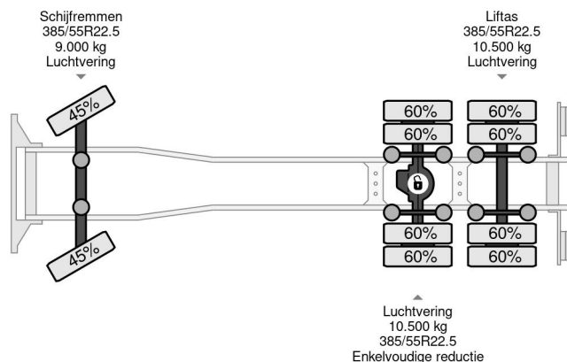
Scania R560 V8 | BERTHONS HOT ROD | CUSTOM S... 6x2
