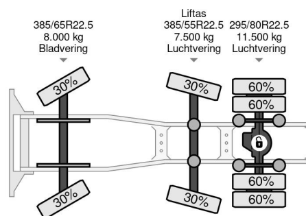
Mercedes-Benz Actros 2545 | 6X2*4 | STEERING AXLE | MI...
