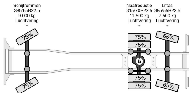
Volvo FH 16.750 | 6X2*4 | EFFER 215 | 6X EXT | RETARDER ...
