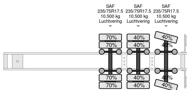
Max Trailer MAX 100 | 3-AXLE | LIFT DECK | SLIDING RAMPS
