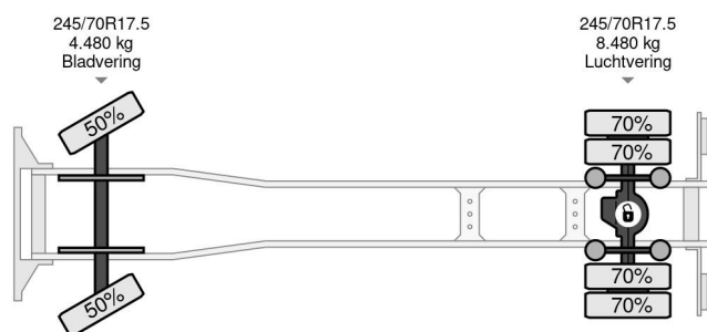
DAF LF 210 FA 4X2 | FALKOM | ABSCHLEPP | 2X WINCH | ...
