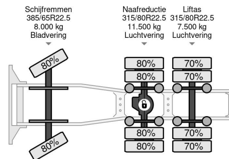
Volvo FH 16.750 6X2 HUB REDUCTION RETARDER SPECIAL
