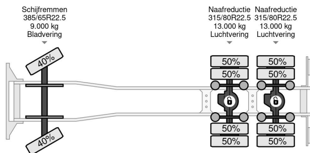
Volvo FH 16.700 | TRACTOR & TIPPER | RETARDER |... 6x4
