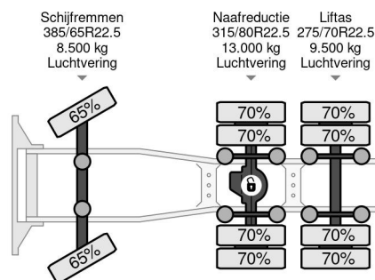
Volvo FH 16.650 6X2 | RETARDER | SPECIAL BUILT | SPEC...
