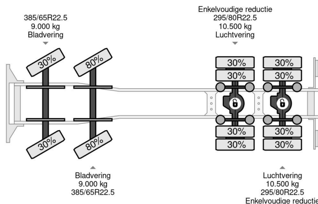
Scania R164-480 V8 8X4 | FASSI F600 | JIB | KRAN / CRANE
