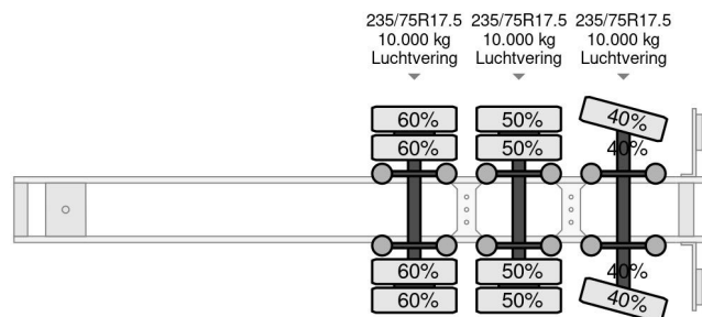
Nooteboom OSDS-48-03-V | 6-MTR EXTENSION | WINCH | ...
