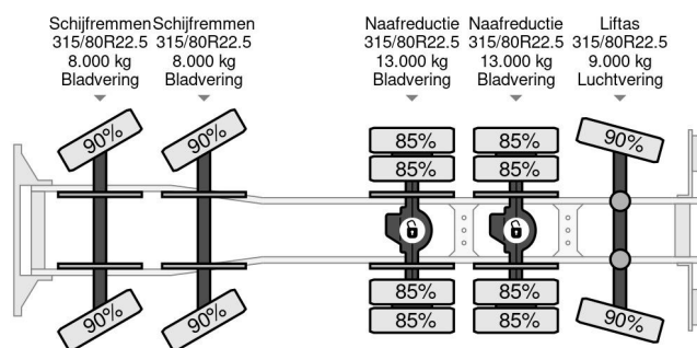
MAN TGS 50.440 | 10X4*6 | SARAKA 28 METER | 8M3 MIXER
