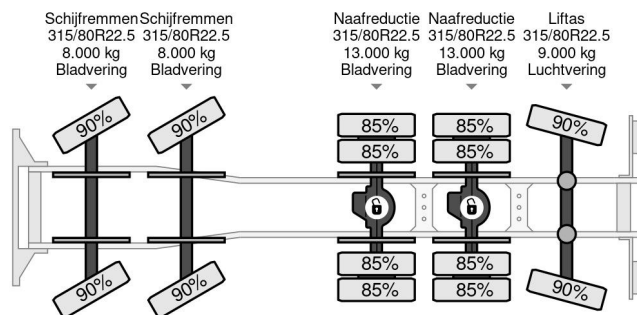
MAN TGS 50.440 | 10X4*6 | SARAKA 28 METER | 8M3 MIXER
