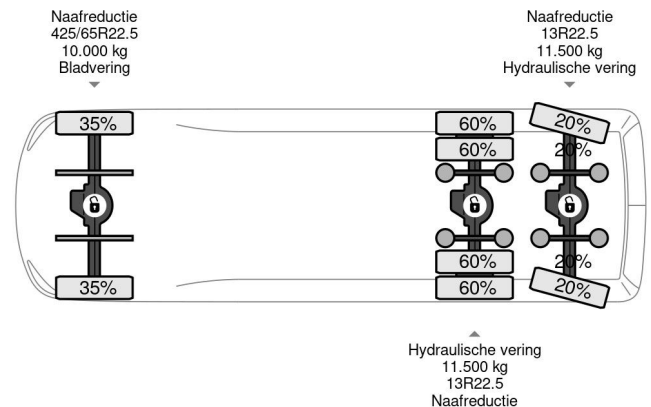
MAN TGS 33.440 6X6 | 2 SIDE TIPPER | ATLAS 165.2 | GR...
