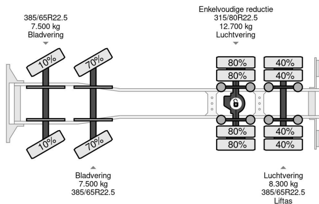
Scania R164-580 V8 8X2 | COPMA 990 | JIB | 6+4 EXT | WI... Referentienummer: 113688
